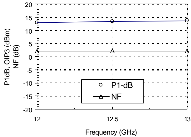
P1-dB and Noise Figure at 25 °C
