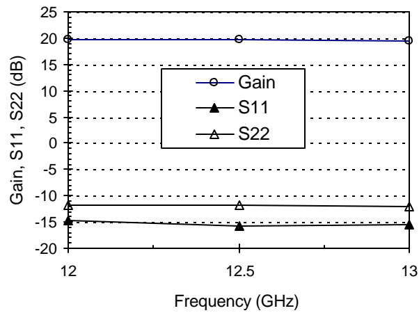
Gain and Return Losses at 25 °C
